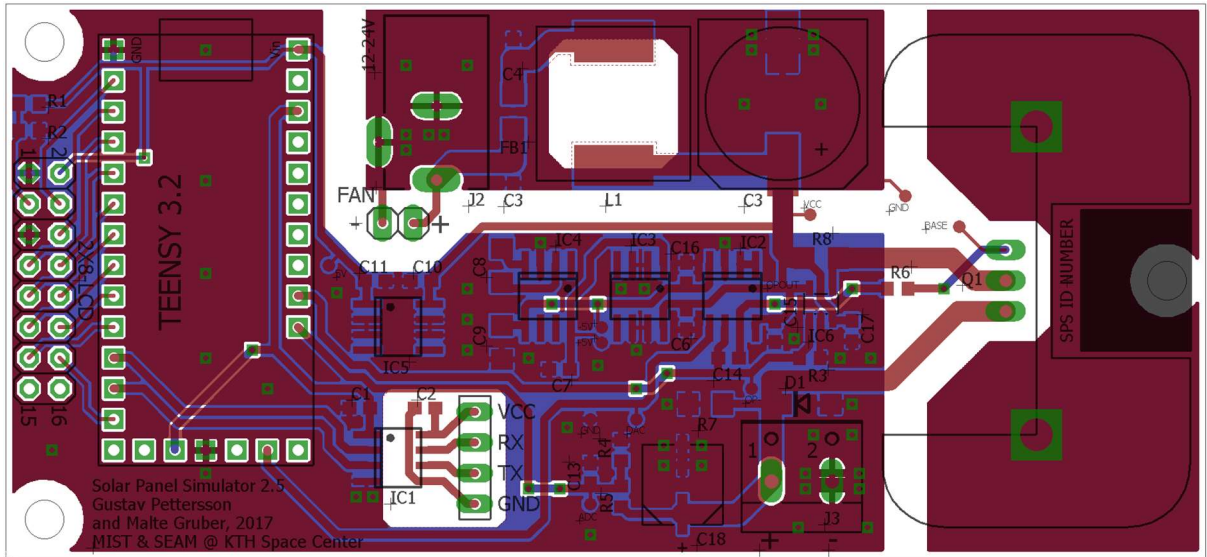
Top, bottom, pads, vias, silkscreen
